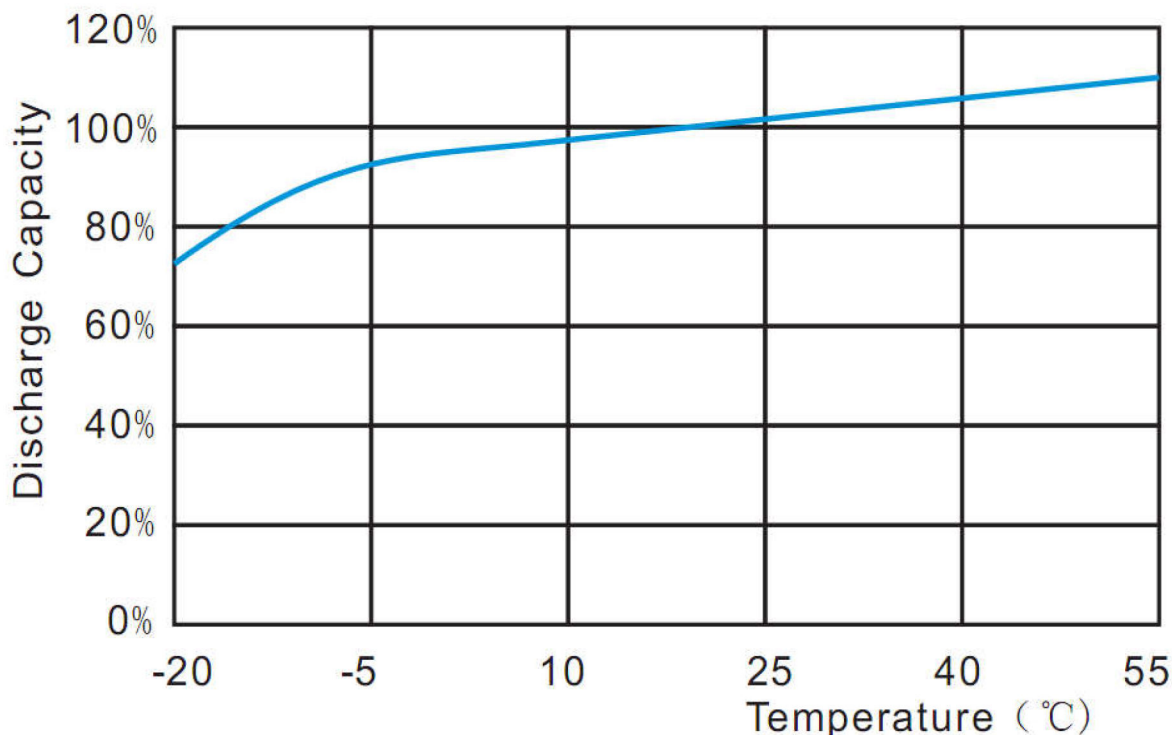
■ Figure 3-1 LC+ Series temperatur effect on battery capacity curve
