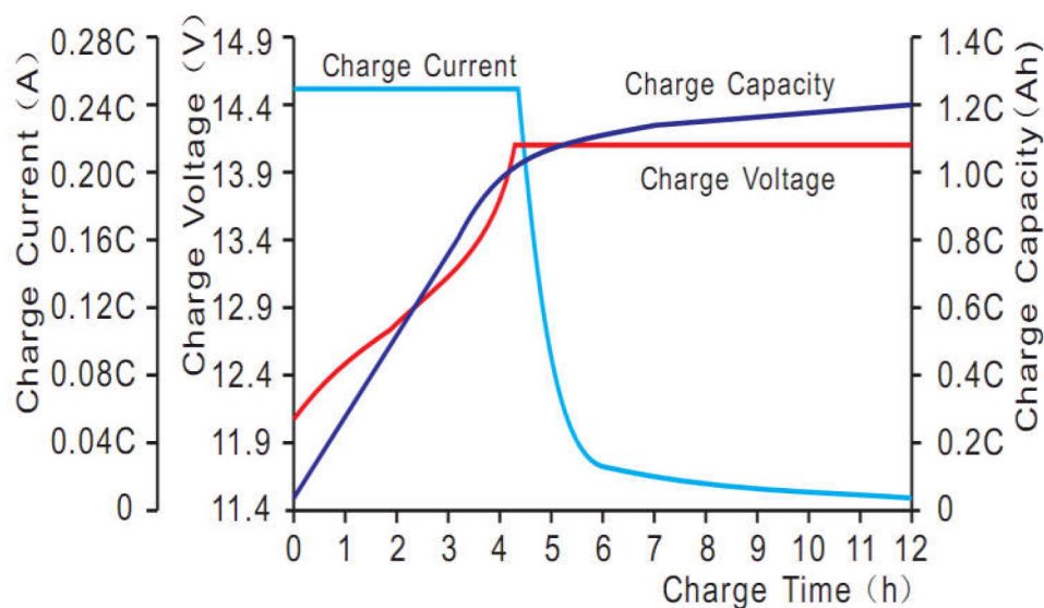
■ Figure 2-2 Charge characteristic curve
